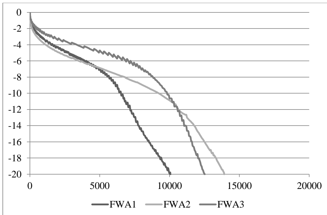
Figure 4.32: Aged field mixed WMA rut depth VS wheel passes
