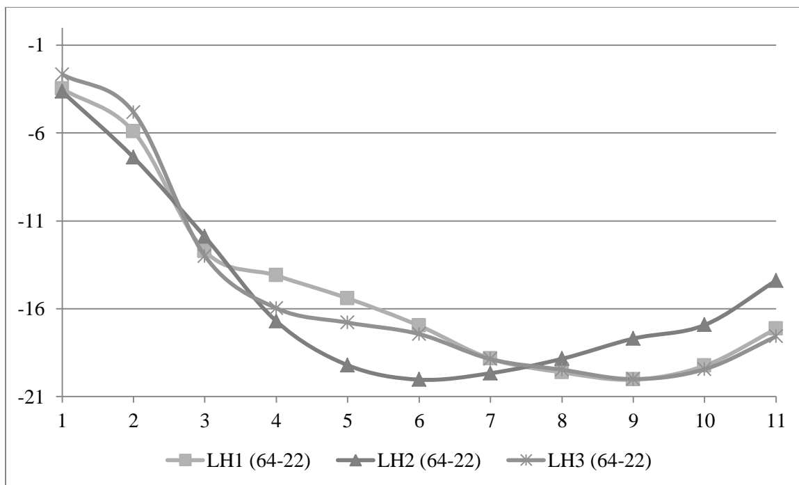
Figure 3.29: Lab Mixed PG 64-22 HMA rut profile
